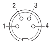
Female 4p molded connector Front View
